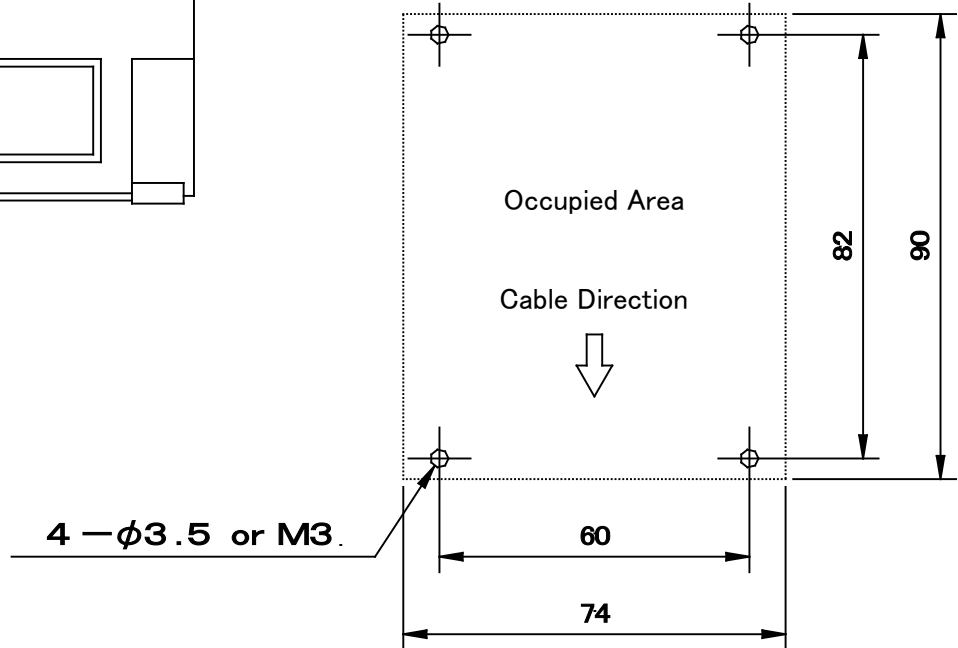
Mounting Pitch Drawing for VM-90A
